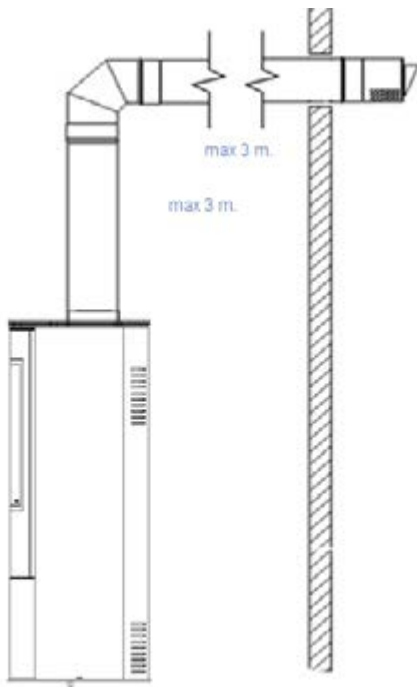
Figure 5. Coaxial system output method
